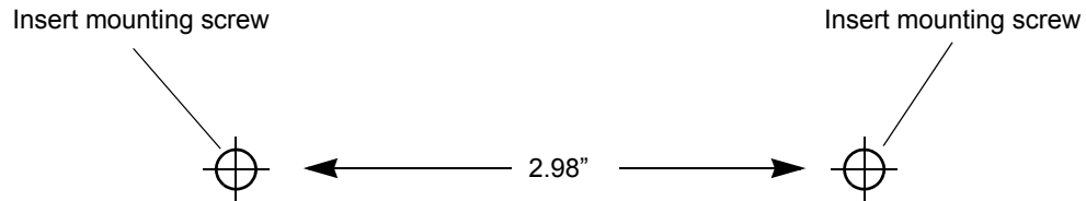
Figure 1-6 Wall Mounting Template
