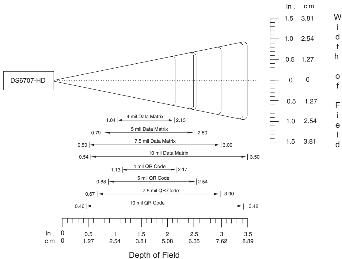
Figure 2-15 Symbol DS6707-HD High Density Digital Imager Scanner Decode Zone for 2D Bar Codes
